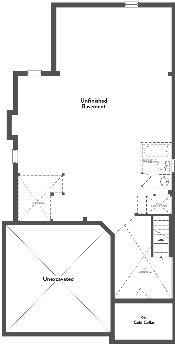
BASEMENT ELEVATION A/B/C 2535/2552 sf
