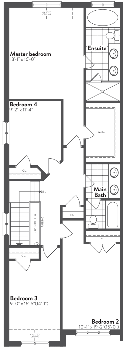
SECOND FLOOR ELEVATION A 2278 sf
