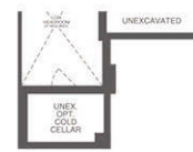
UNFINISHED BASEMENT/ 274 OF OPT. FINISHED BASEMENT ELEVATION B2 1417/1691 sf
