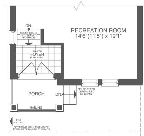
ELEVATION B LOWER FLOOR
