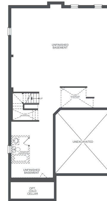
ELEVATION C BASEMENT
