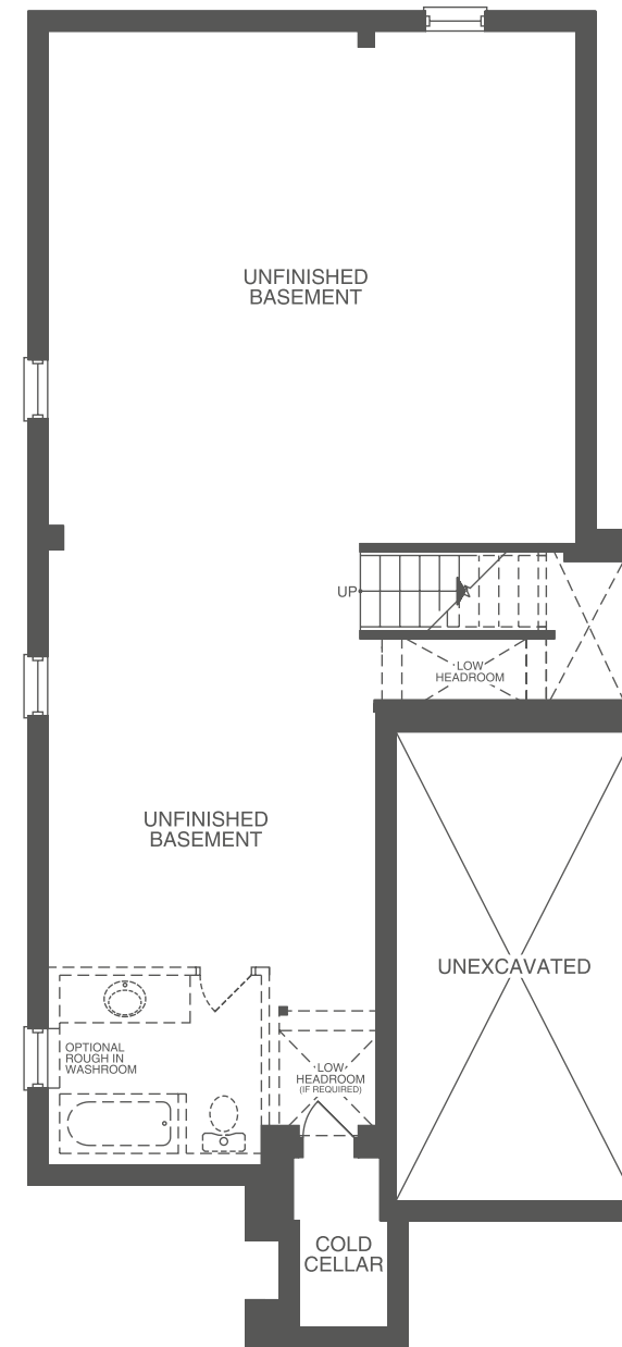
ELEVATION A & B BASEMENT
