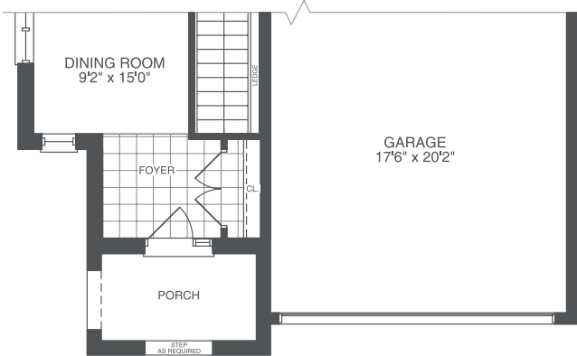
ELEVATION B FIRST FLOOR
