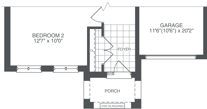
ELEVATION B FIRST FLOOR
