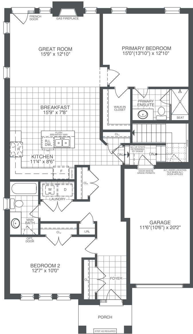
ELEVATION A FIRST FLOOR
