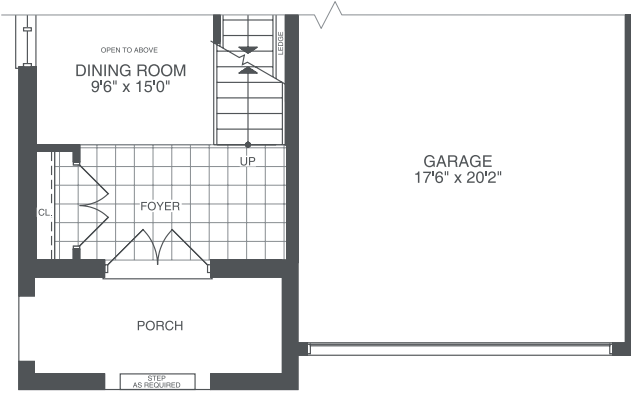
ELEVATION D FIRST FLOOR
