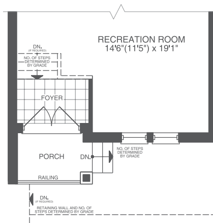
ELEVATION B LOWER FLOOR
