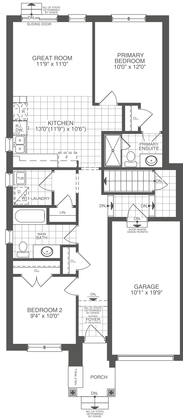
ELEVATION A & B FIRST FLOOR
