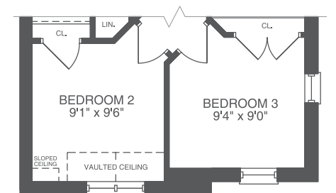
ELEVATION B UPPER FLOOR
