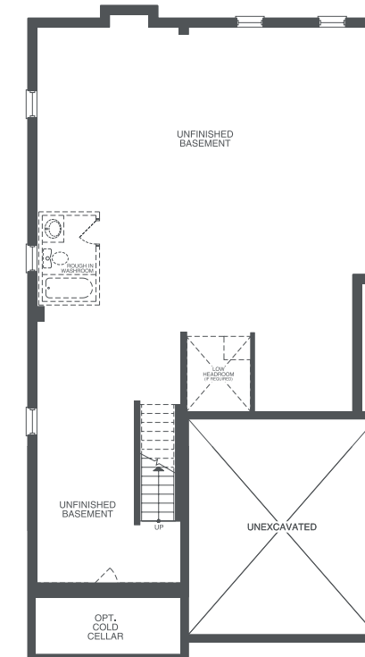
ELEVATION C & D BASEMENT
