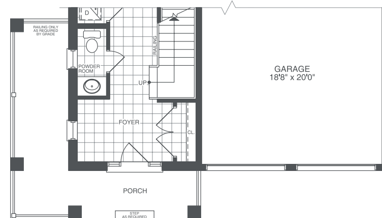
ELEVATION D FIRST FLOOR
