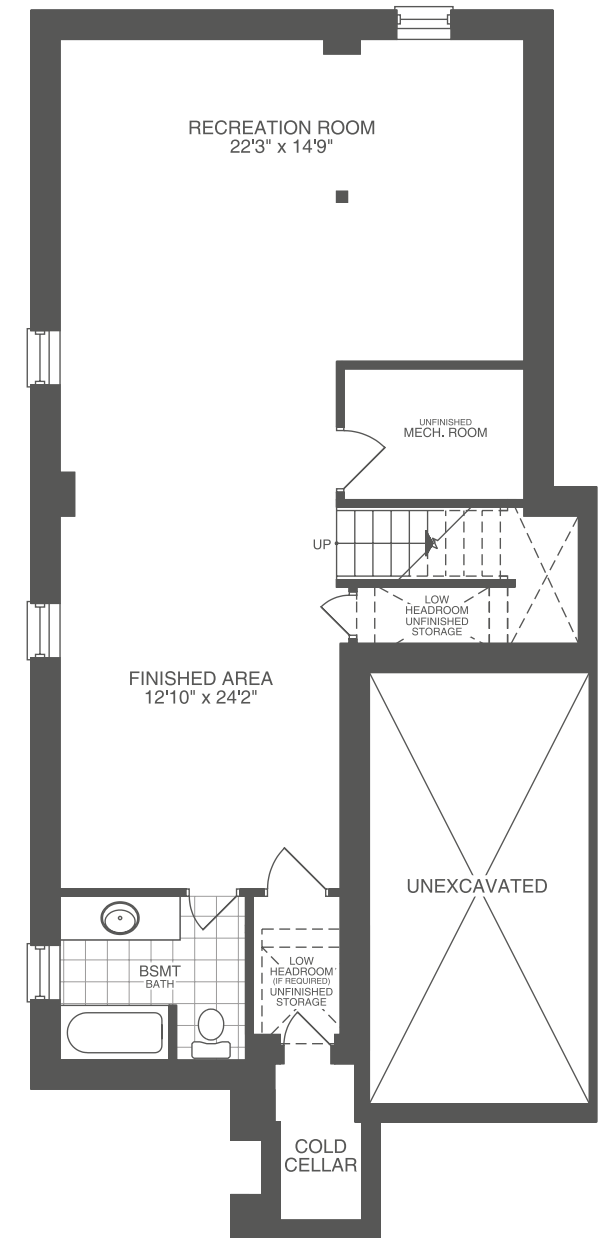
ELEVATION A & B OPT. FINISHED BASEMENT
