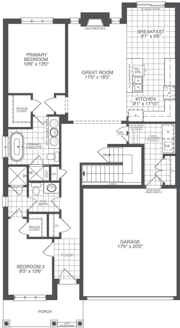
ELEVATION A FIRST FLOOR
