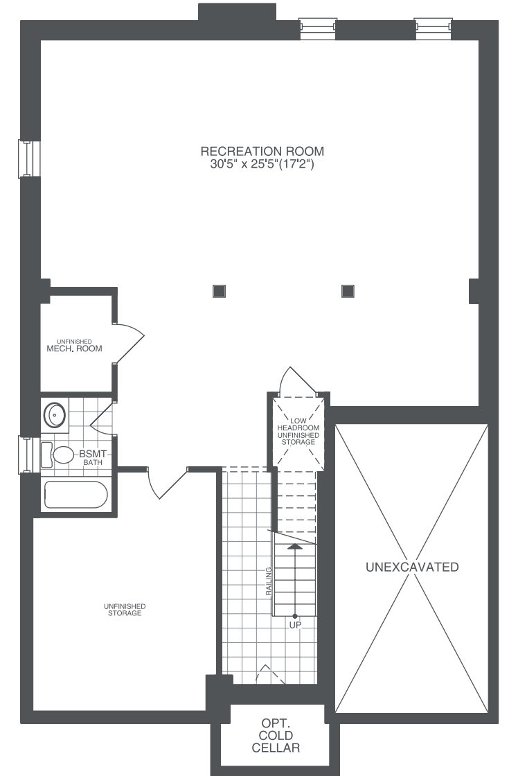
ALL ELEVATIONS OPT. FINISHED BASEMENT
