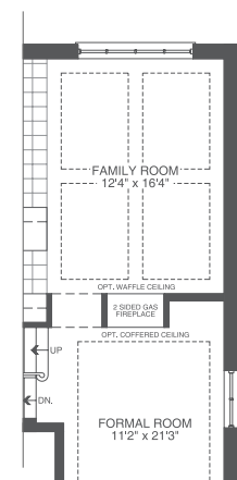
GROUND FLOOR OPT. FIREPLACE
