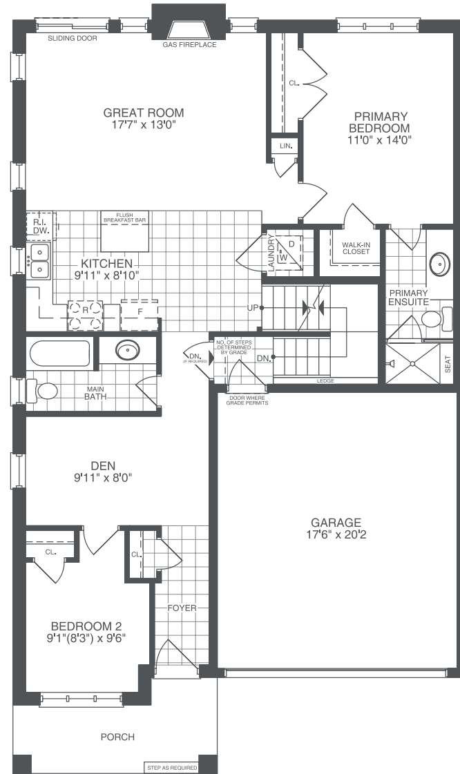
ELEVATION C FIRST FLOOR
