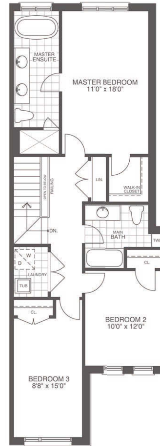
SECOND FLOOR PLAN ELEVATION A 1715 sf
